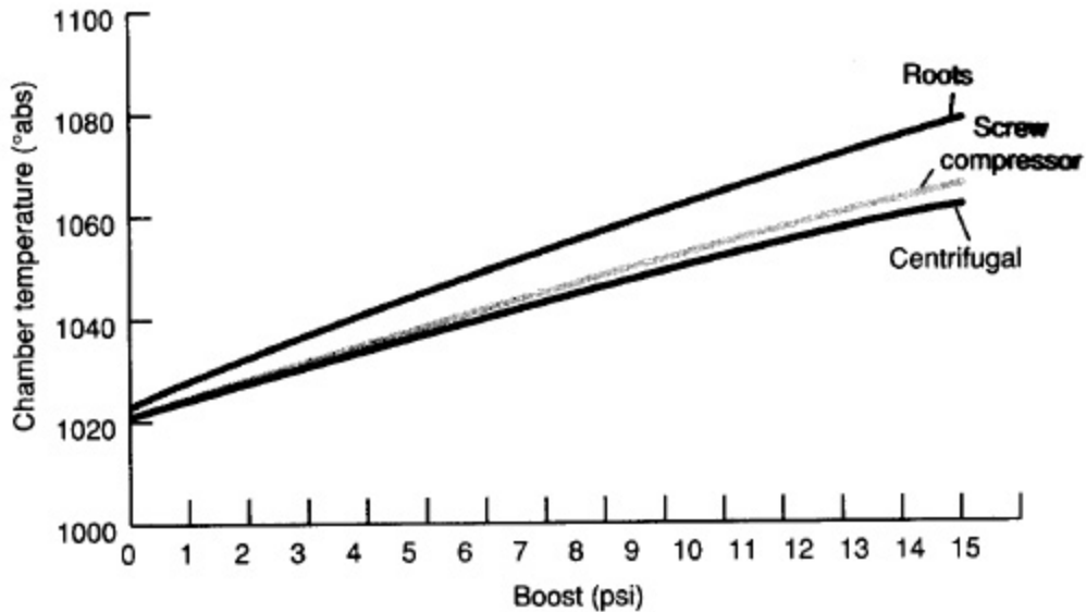
Fig. 4-4: Chamber temperature gain after intercooling, as a function of boost for a 9-to-1 compression ratio. These temperatures are found by using the numbers from Fig. 4-3 (and ambient temperature of 90°F) in the temperature formula.
