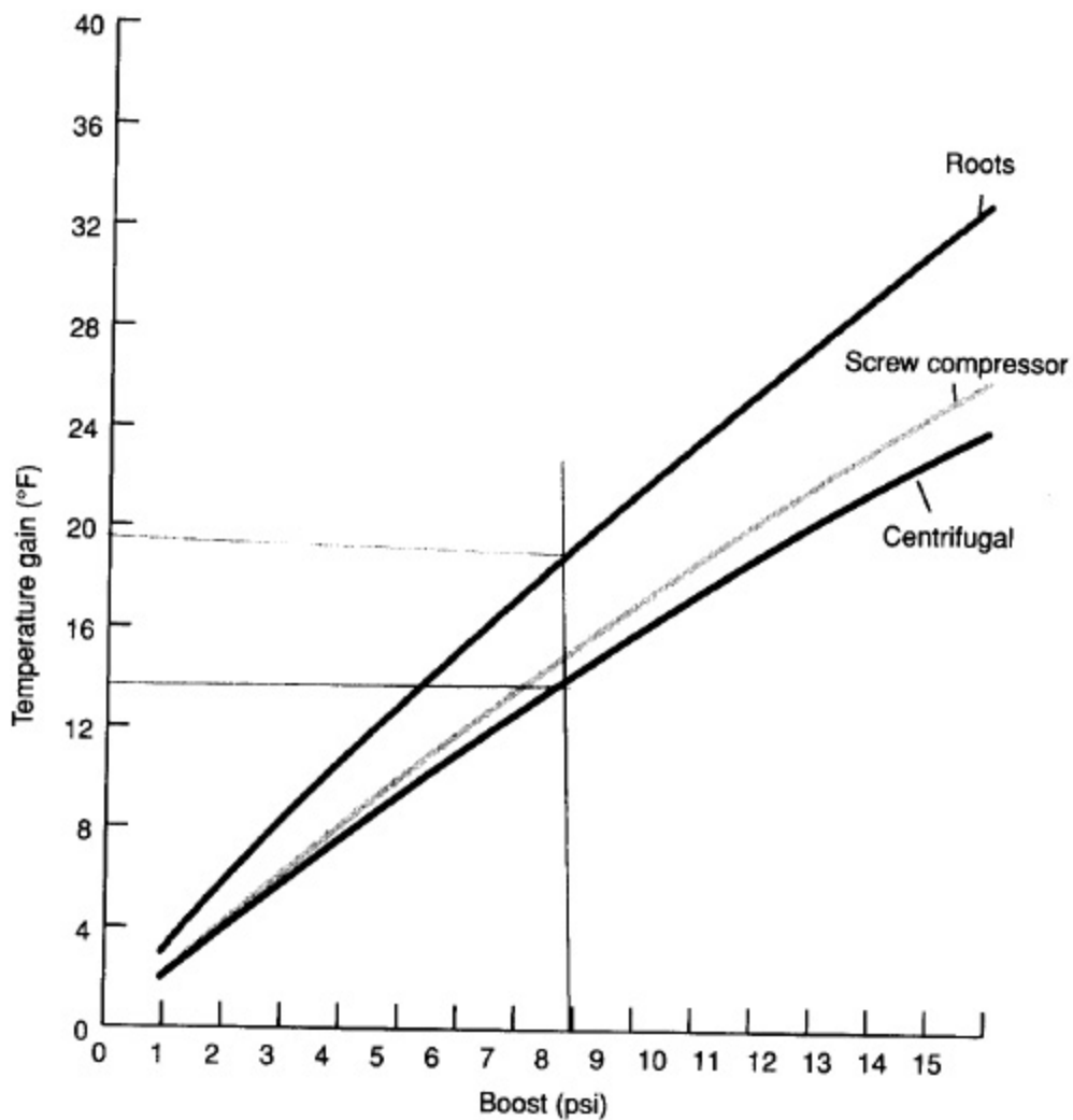
Fig. 4-3: Compressor discharge temperature gain after intercooling, as a function of boost.
