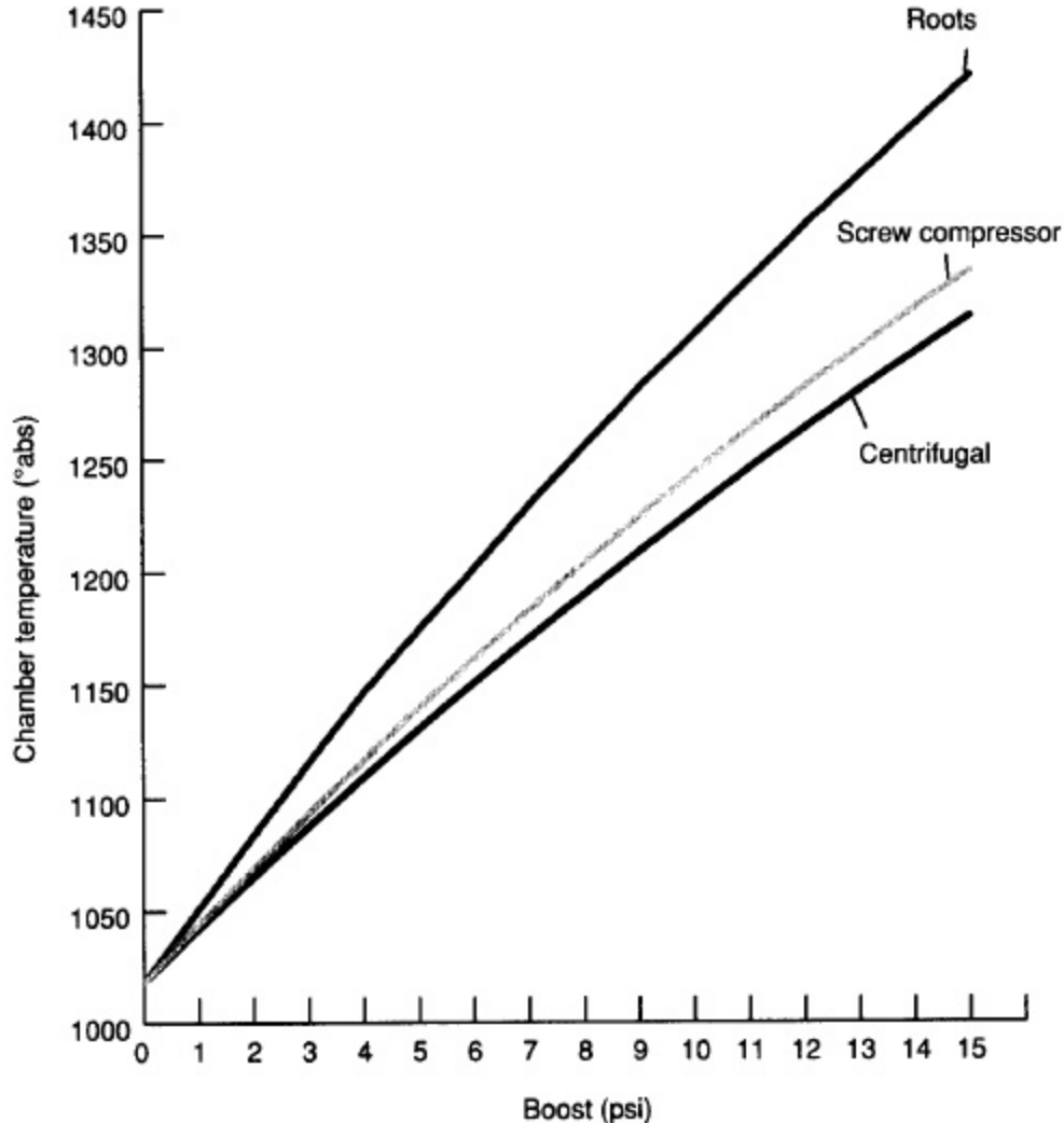
Fig. 4-2: Chamber temperature gain as a function of boost for a 9-to-1 compression ratio. These temperatures are found by using the numbers from Fig. 4-1 (and ambient temperature of 90°F) in the temperature formula.
