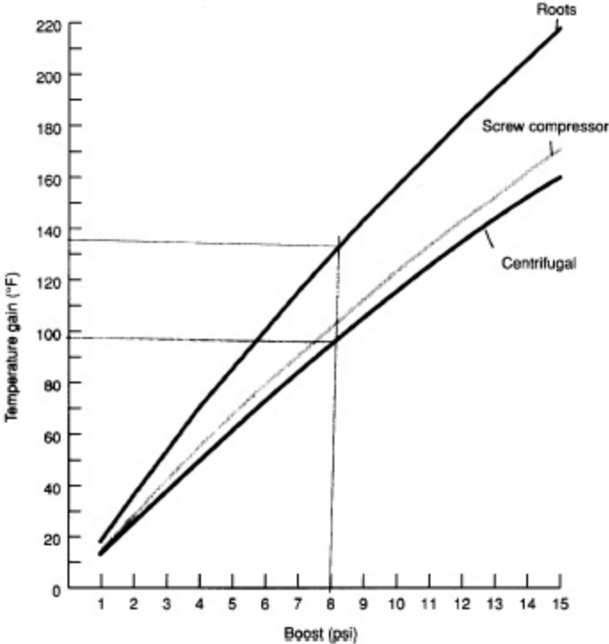
Fig. 4-1: Compressor discharge temperature gain as a function of boost.
